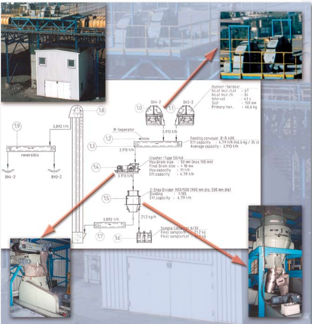
Automatic sample taking and preparation system for coal, train unloading, Qinhuangdao, China Project management in cooperation with our sister company TEMA B.V.
