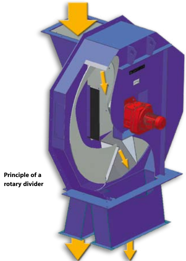
Rotary divider
