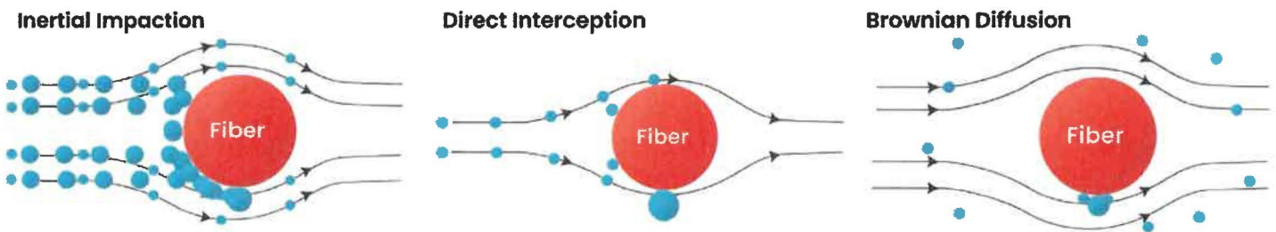
Mechanisms for mist collection on fibers.
