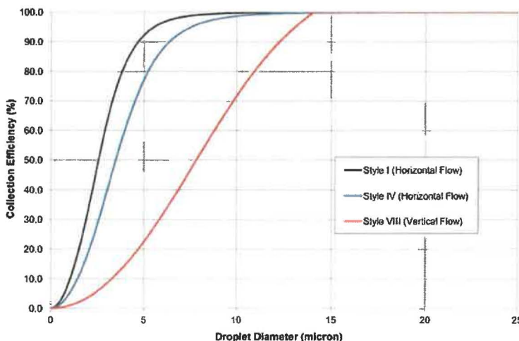
Typical collection efficiency vs. droplet size of a FLEXICHEVRON® mist eliminator in air-water system at atmospheric conditions.
